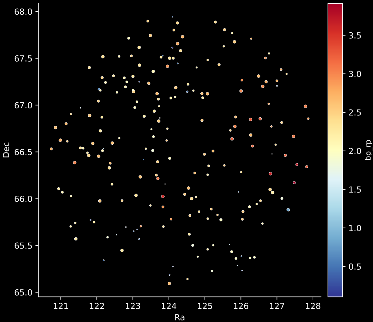
APOGEE DR17 Field: [128+04] Stars: 206
