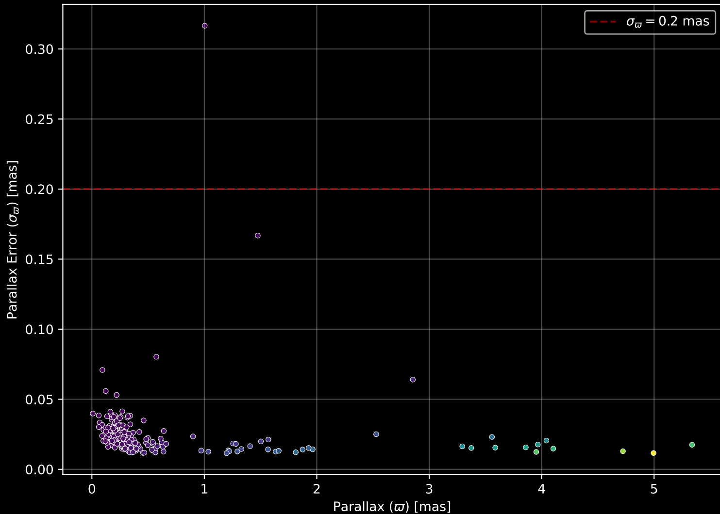
APOGEE DR17 Field: [128+04] Parallax Quality (n= 206)
