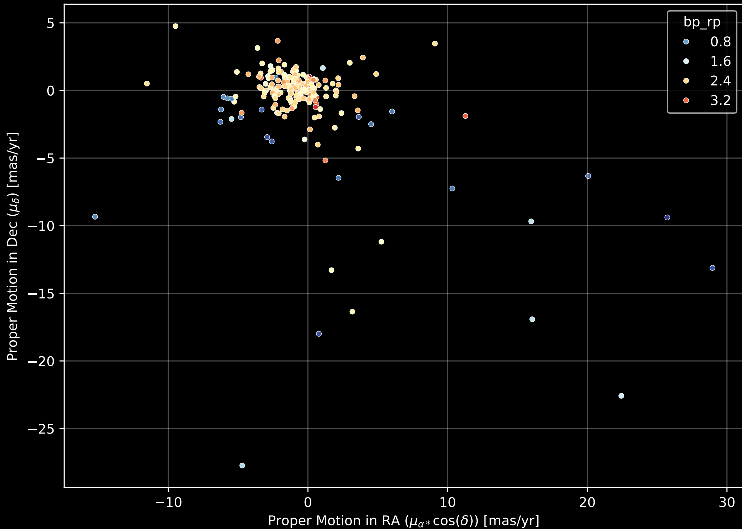
APOGEE DR17 Field: [128+04] Proper Motion Diagram (n= 206)
