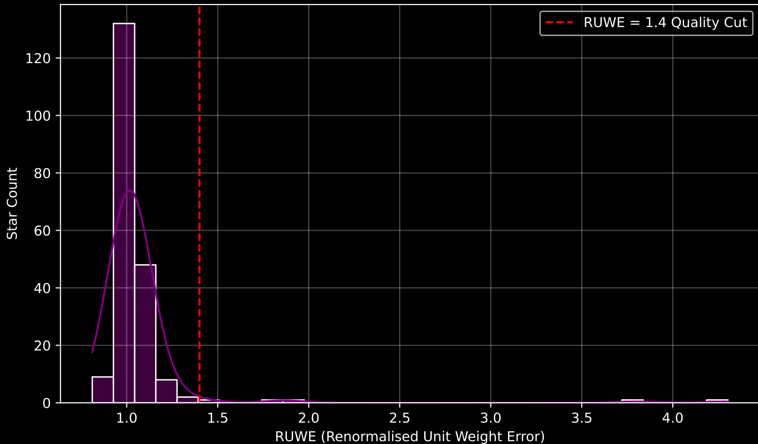
GAPOGEE DR17 Field [128+04] RUWE Distribution (n= 204)
