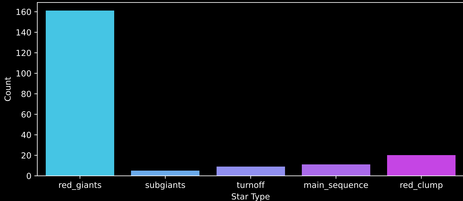
APOGEE DR17 Field: [128+04] Count plot of Star Type
