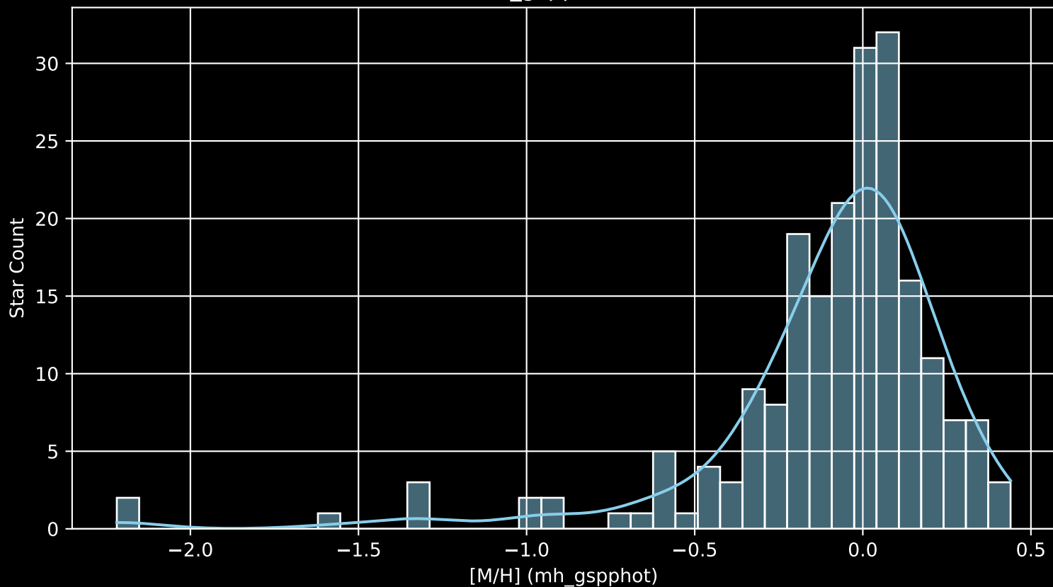
APOGEE DR17 Field: [128+04 [M/H] (mh_gspphot) (n= 204)
